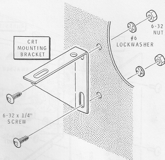
Detail 5-4C
