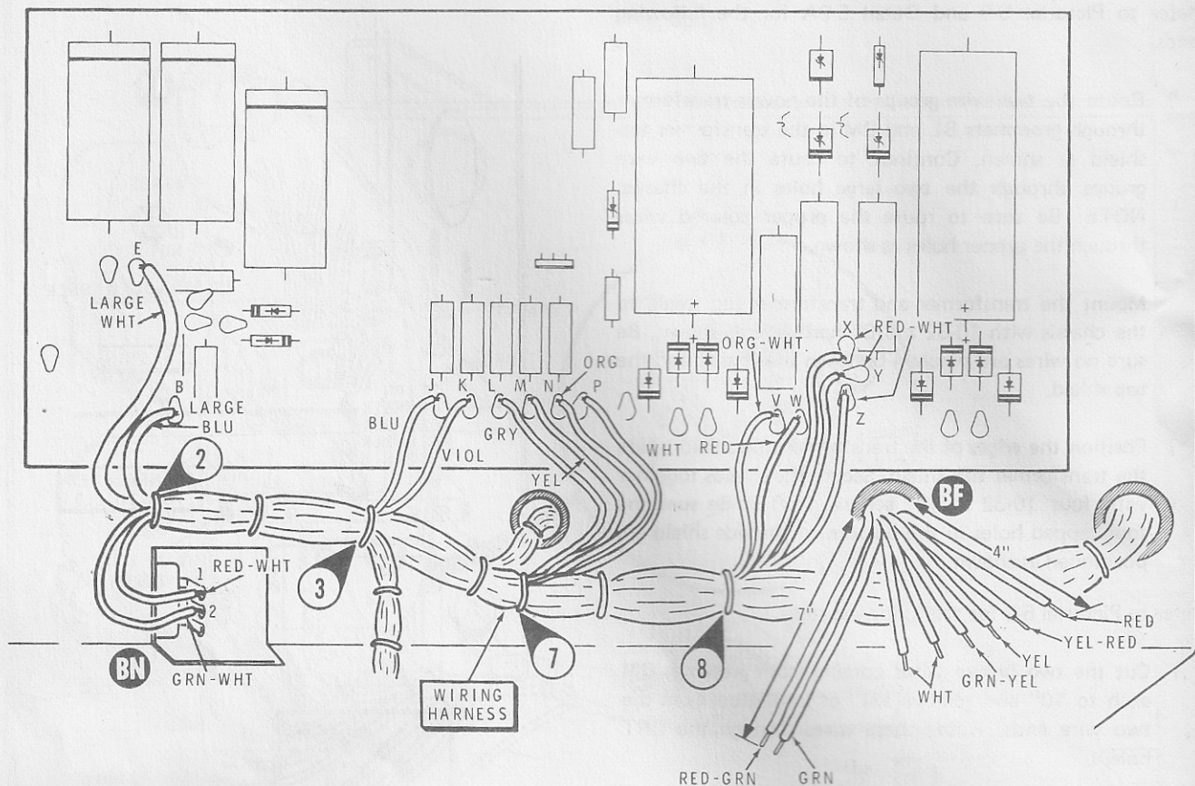
PICTORIAL 5-10
