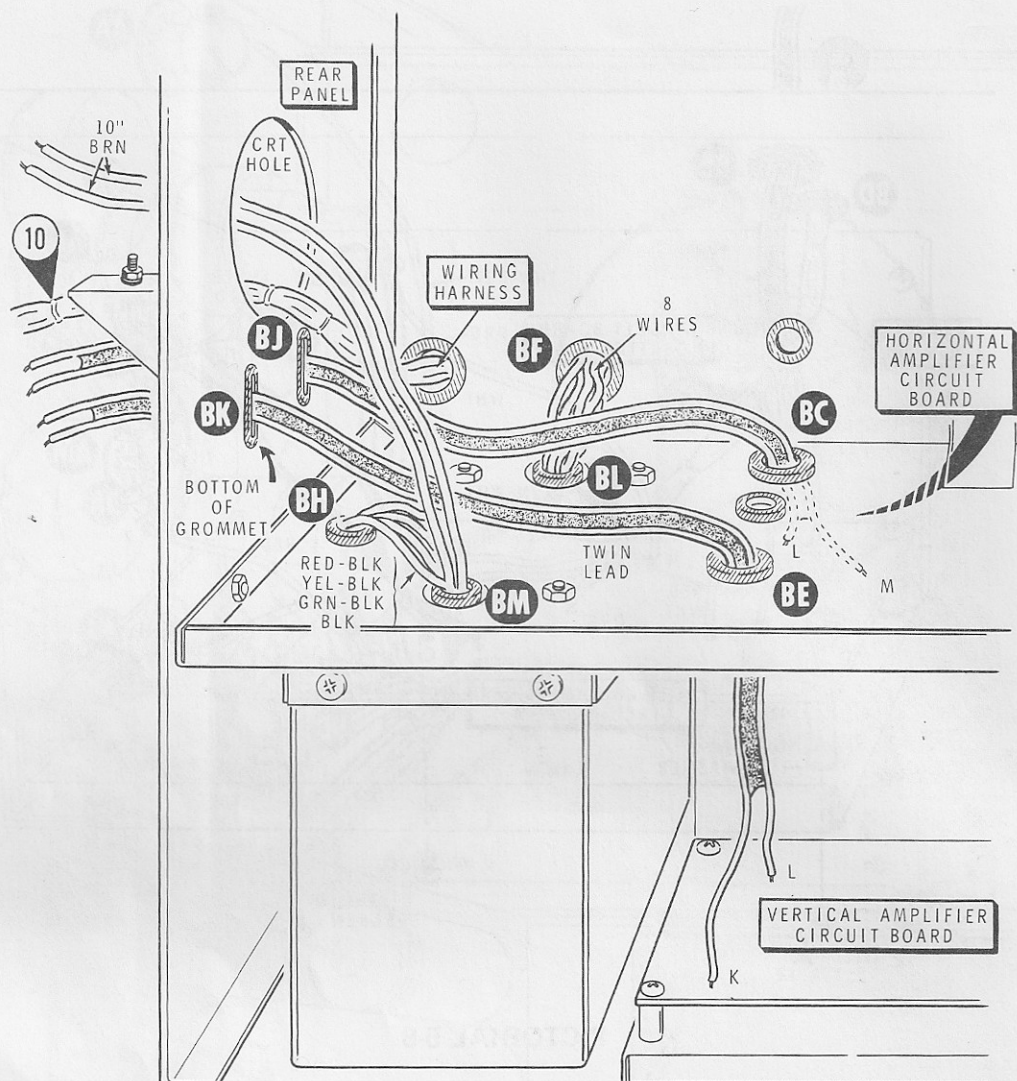
PICTORIAL 5-9
