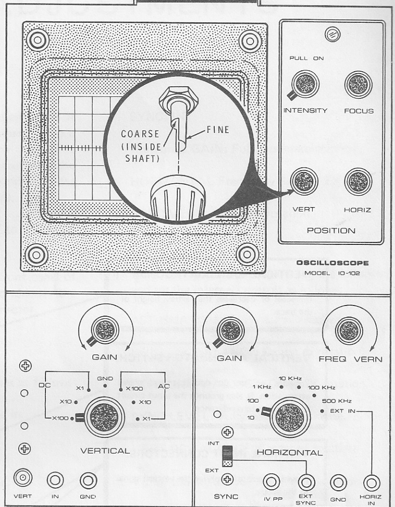
PICTORIAL 5-15
