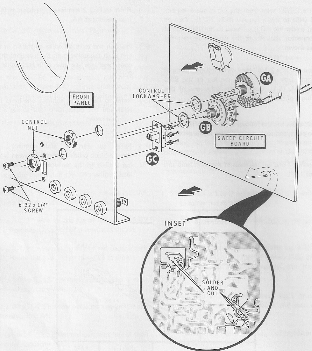
PICTORIAL 5-3
